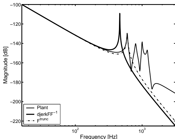
Fig. 8. Plant and inverse of feedforward controllers. Plant (solid thin), Mode inversion based feedforward controller (dashed), derivative of jerk feedforward controller (solid thick).
