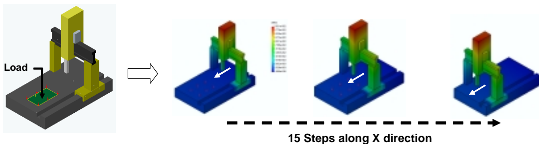
Figure 2 – Path of the bridge over a deformed granite table
