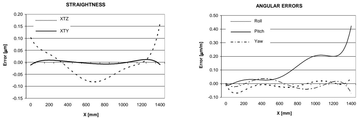
Figure 3 – Linear and Angular Errors of the machine bridge along its path
