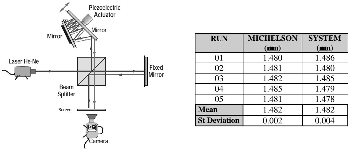
Figure 2 – Calibration with a modified michelson intereferometer
