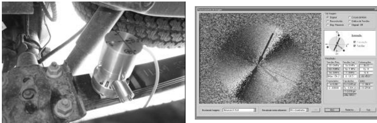
Figure 3 – Optical Rousette measuring the stress/strain in a truck suspension and a software result
