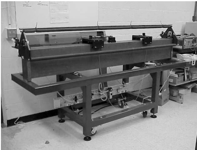
Figure 3. Prototype 1DMM
